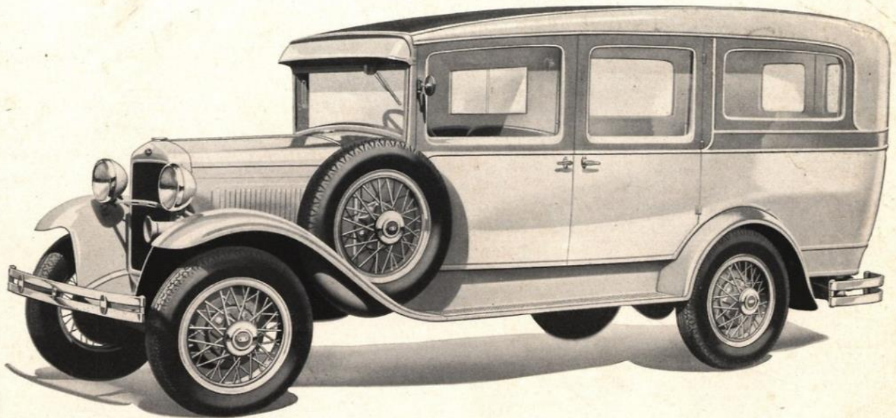
THE FORD AMBULANCE Length, 102"; Height, 55"; Width, 54". Wheelbase, 131½".
